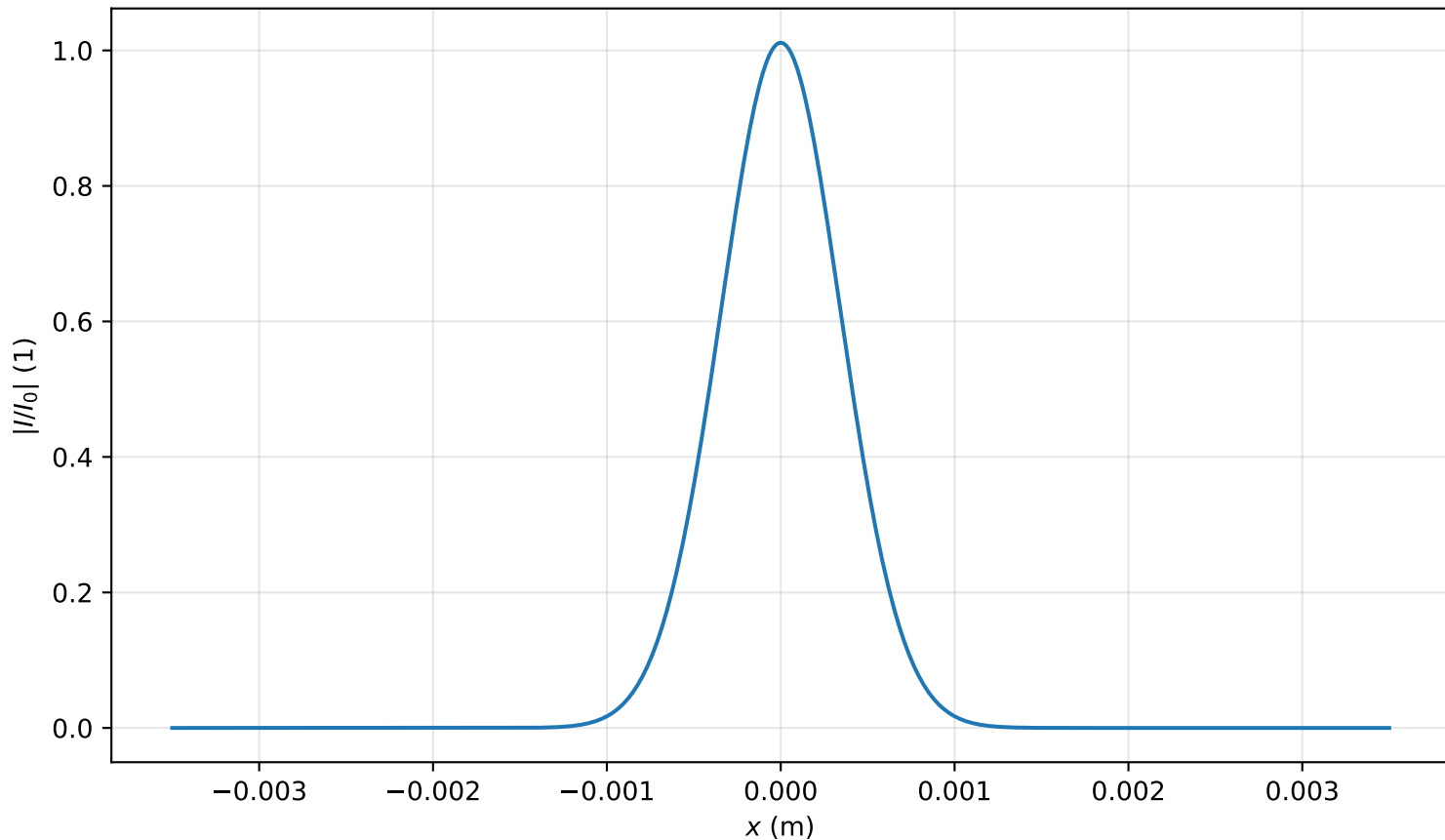
Intensity profile I(x, y = 0, z = 0.159m)/I_0 , P_{in}=0.7P_{cr} , artificial time
